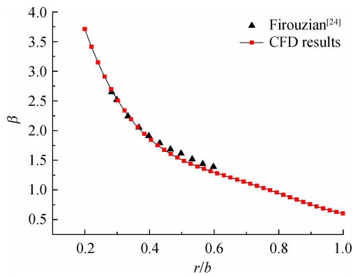
图 4 文献实验数据与仿真数据对比图 [24] Fig. 4 Comparison of experimental and CFD results [24]
